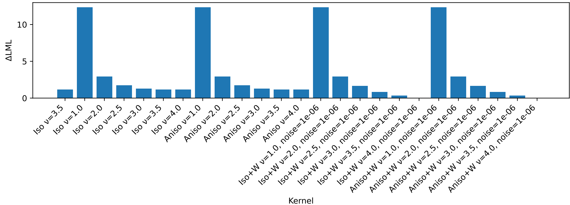
Difference from best LML (T23)
