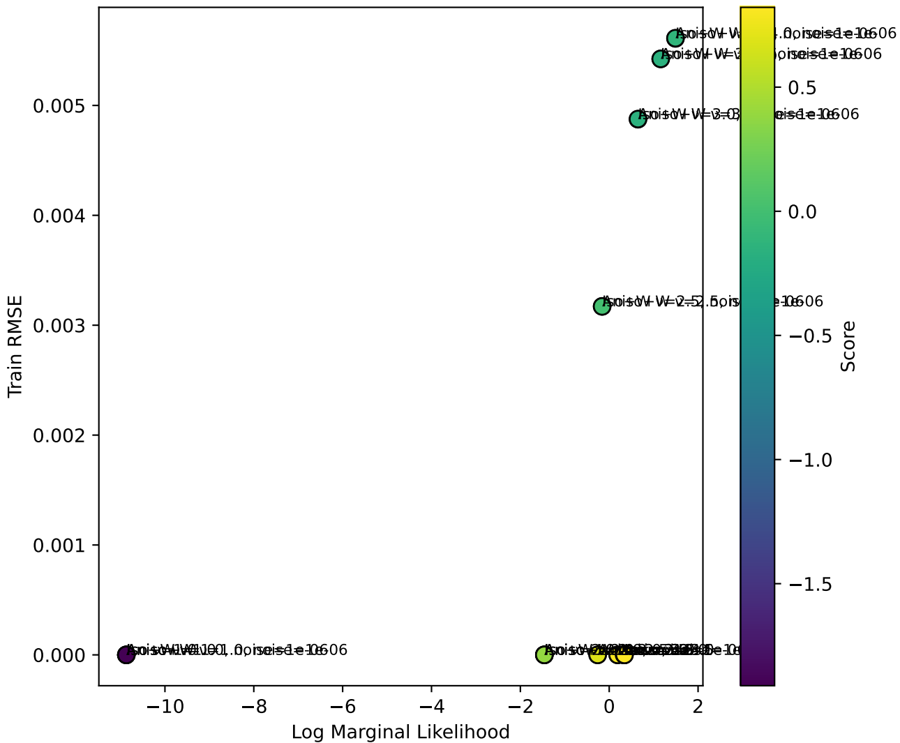
LML vs RMSE (T23)
